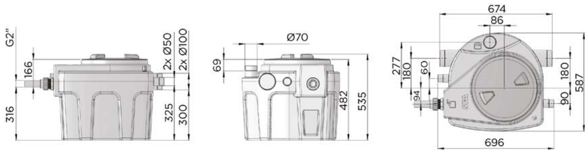
Dimensions (mm)
